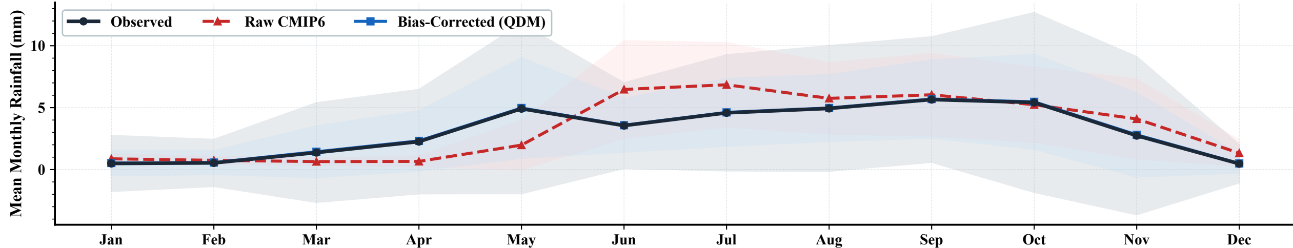
Regional Mean Monthly Climatology ( 1\pm\sigma shading)
